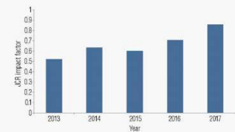
Fig. 1. This graph shows an increasing trend of the impact factor of the InCite Journal Citation Reports (JCR), which was 0.860 in 2017.
